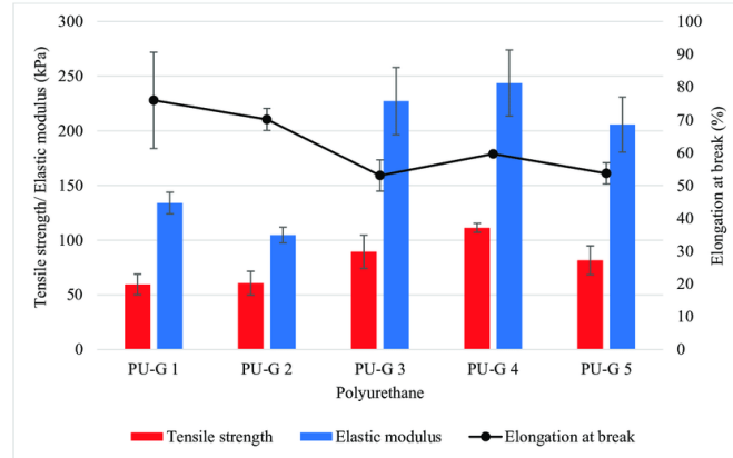
Figure 4-2: Tensile strength of different polyurethanes produced by different water content
