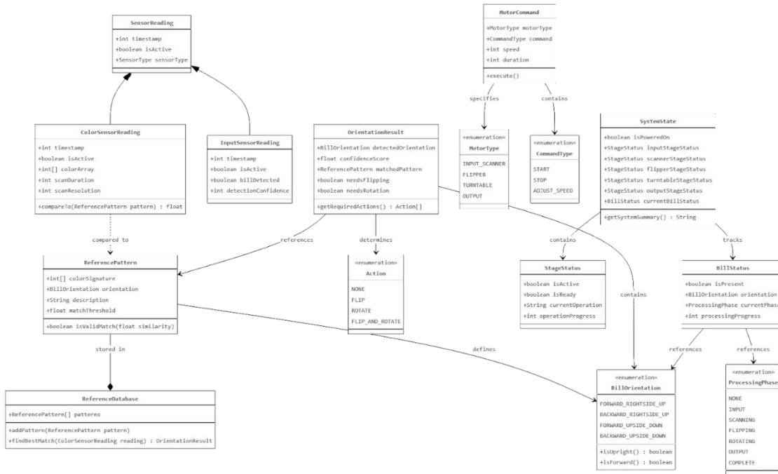
Figure 7-4: Data Structure Diagram
