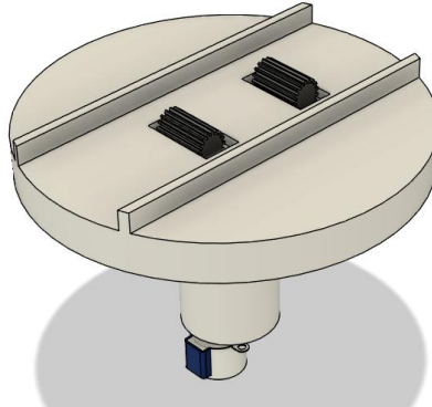
Figure 2-4: Rotating Mechanism
