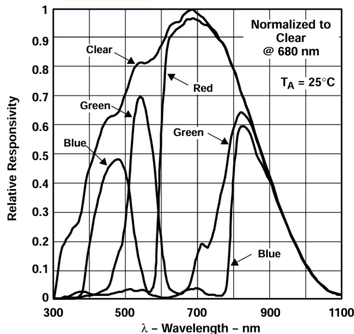
Figure 3-11: Photodiode Spectral Responsivity
