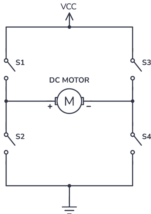
Figure 3-3: Half Bridge Example
