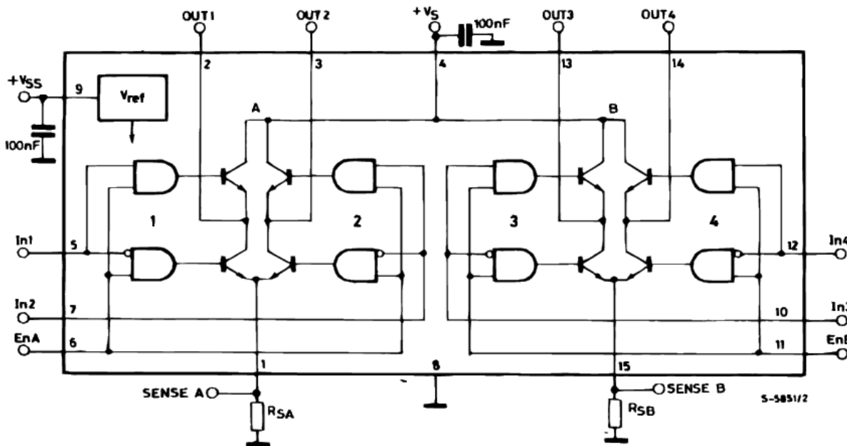
Figure 3-4: Schematic for L298
