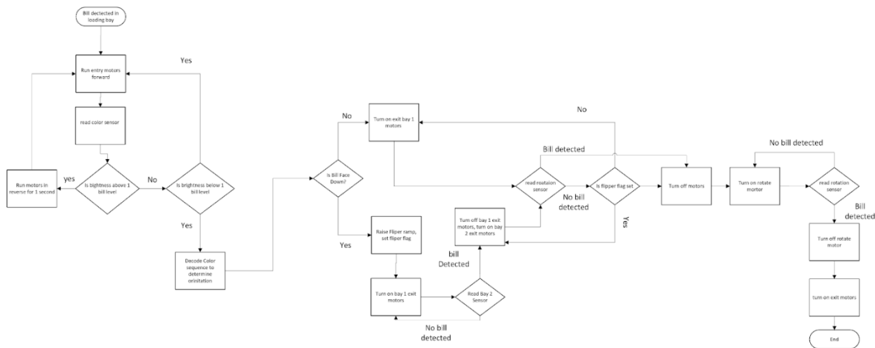
Figure 2-7: Software Flowchart by Authors
