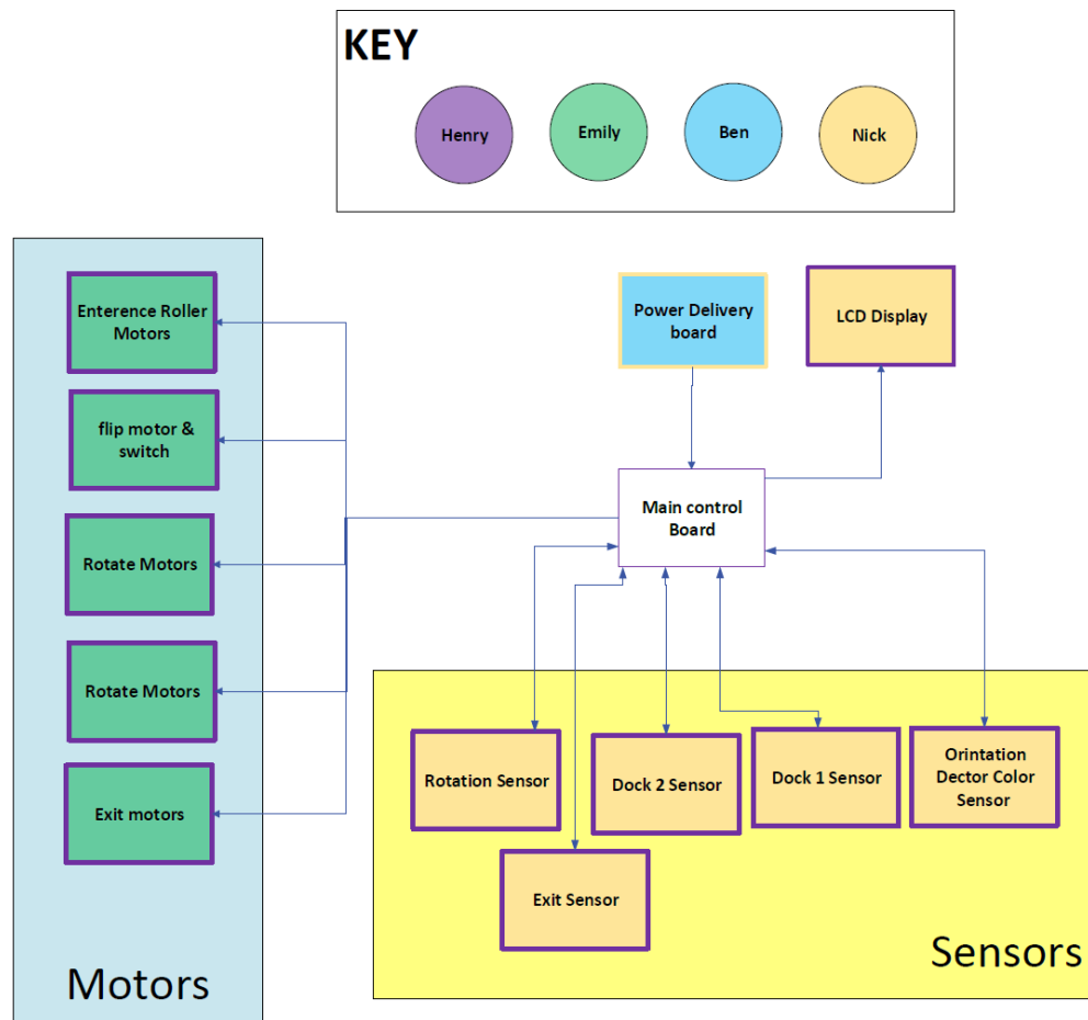
Figure 2-6: Hardware Block Diagram by Authors
